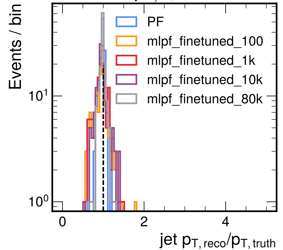
40 < p_{T, \text{truth}} \leq 60
