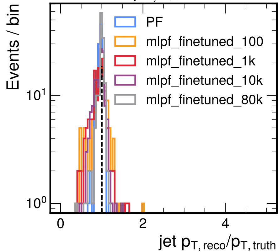
20 < p_{T, \text{truth}} \leq 40
