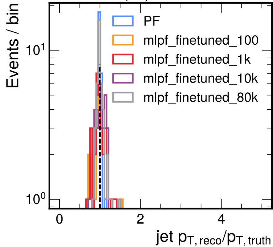
80 < p_{T, \text{truth}} \leq 100
