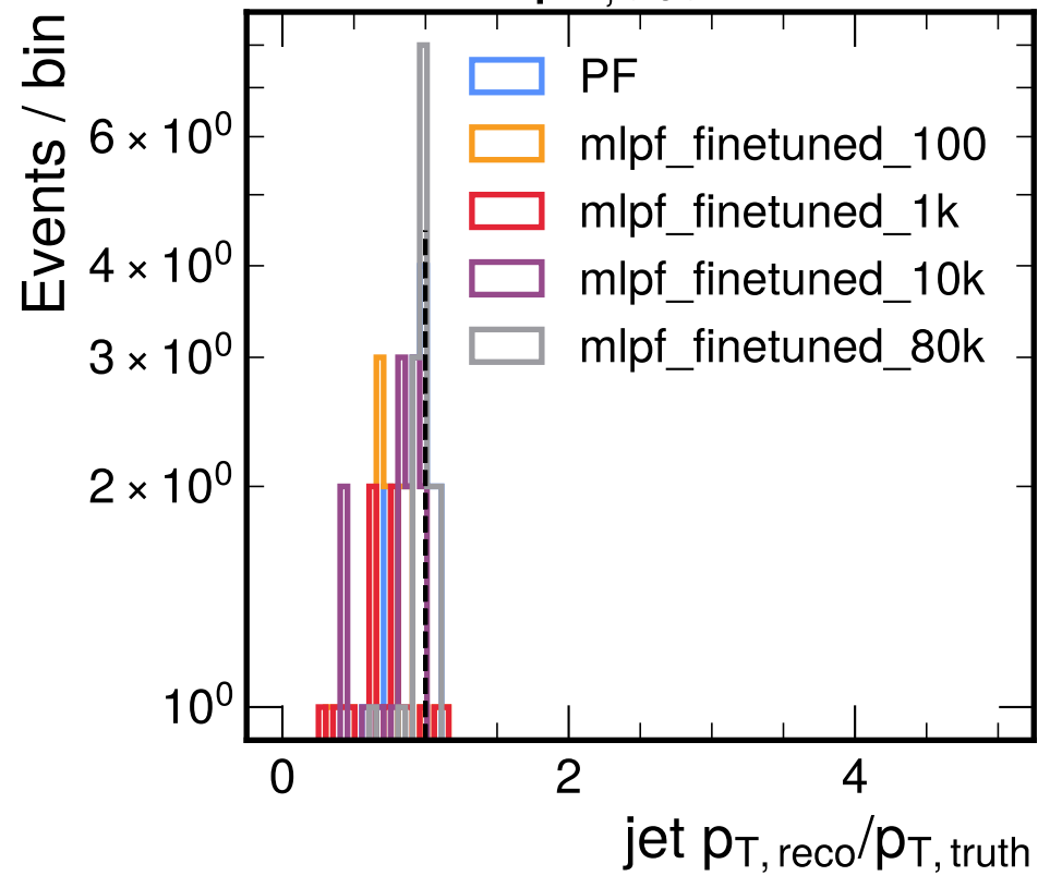
10 < p_{T, \text{truth}} \leq 20
