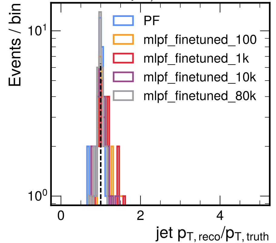
100 < p_{T, \text{truth}} \leq 200
