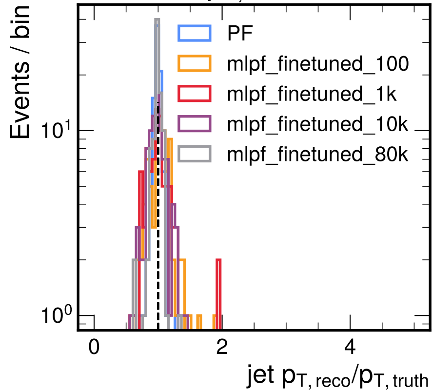
60 < p_{T, \text{truth}} \leq 80
